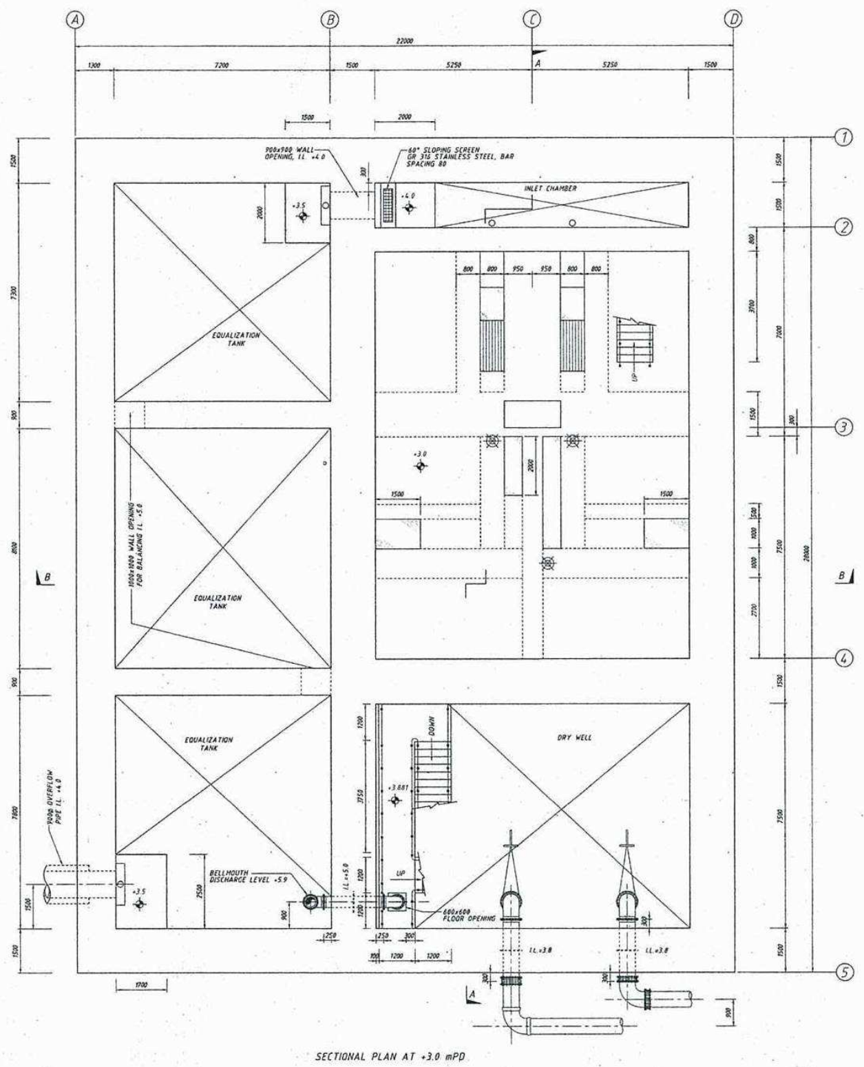
Figure 3: Sewage Pumping Station and Equalization Tanks - Plans
